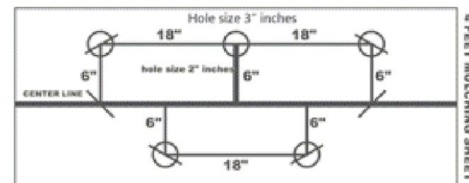
Mulching sheet with zig zag 12x18 hole drawing
